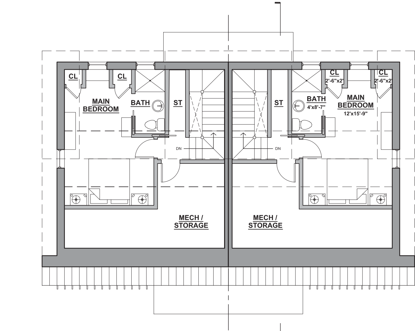
Third Floor Plan 1/8"=1'-0"
