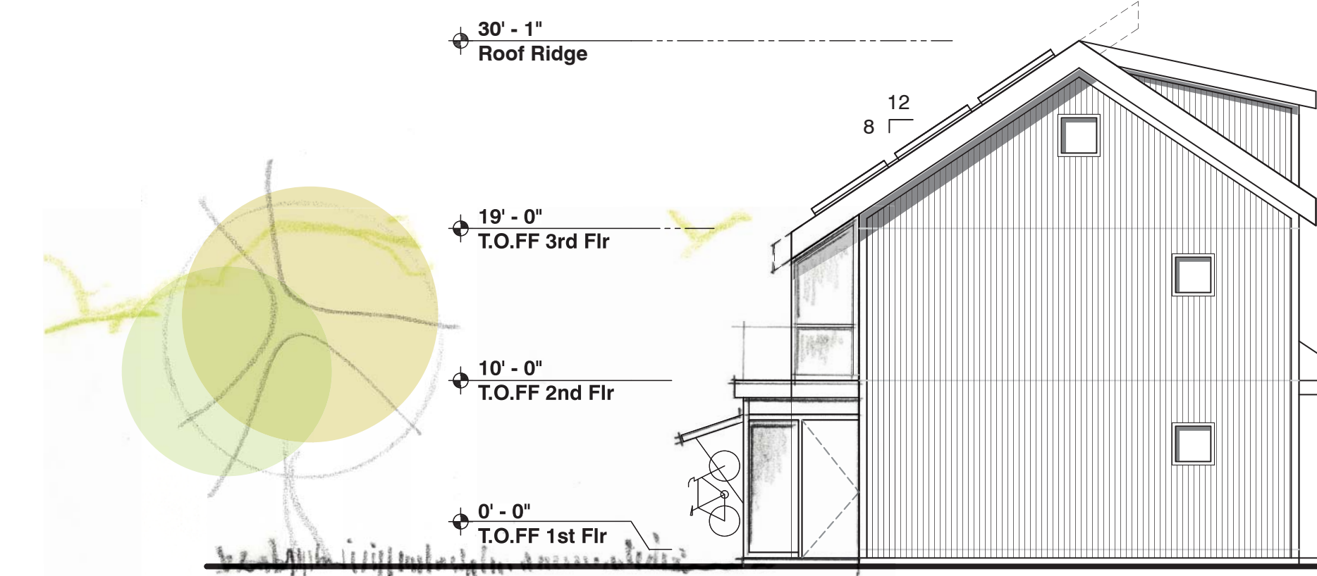
East Elevation _ 1/8"=1'-0"
