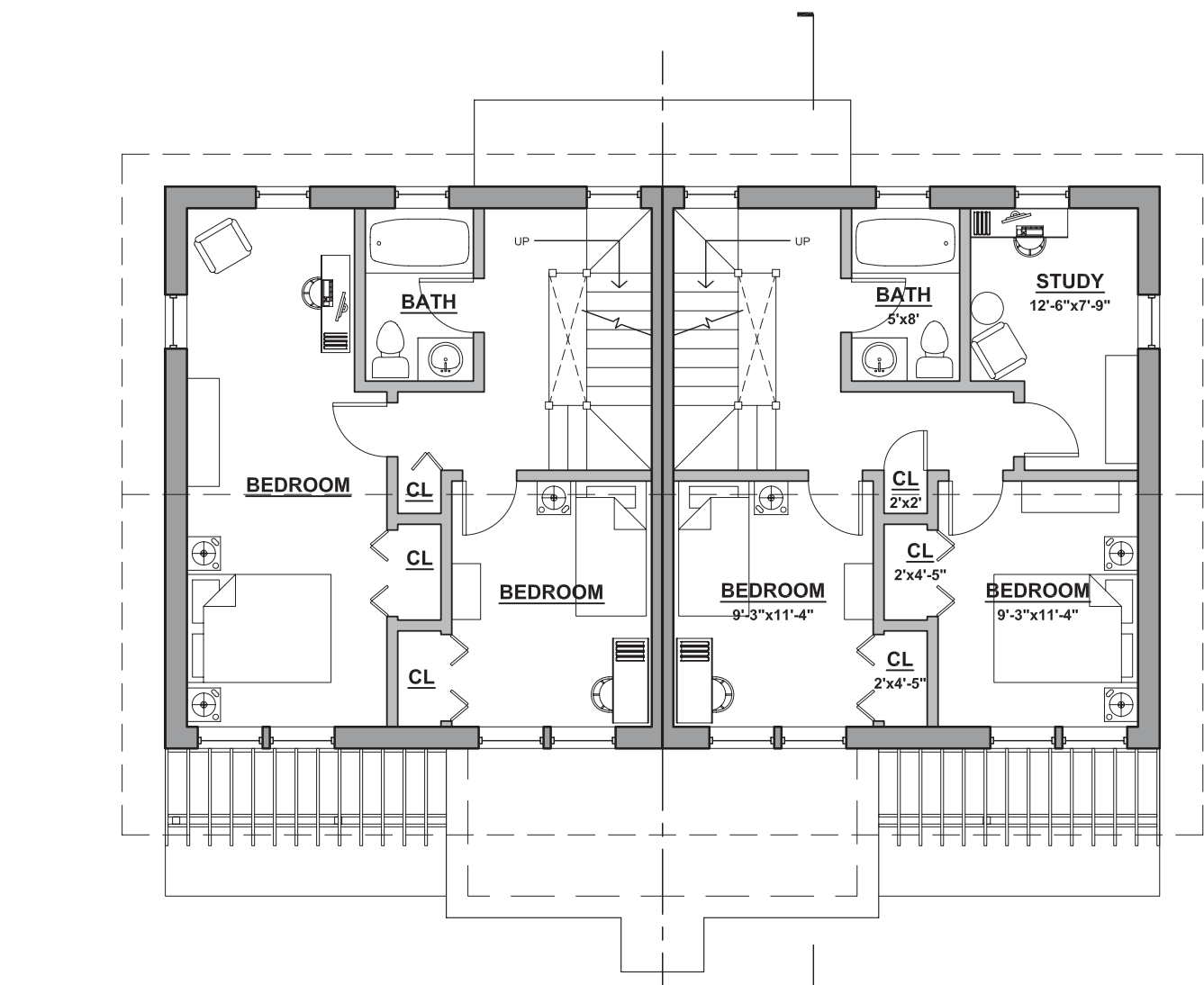
Second Floor Plan 1/8"=1'-0"
