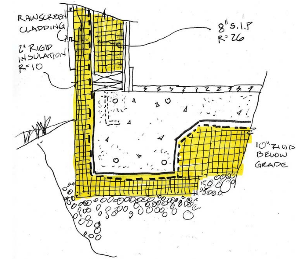
Wall Details 1"=1'-0"
